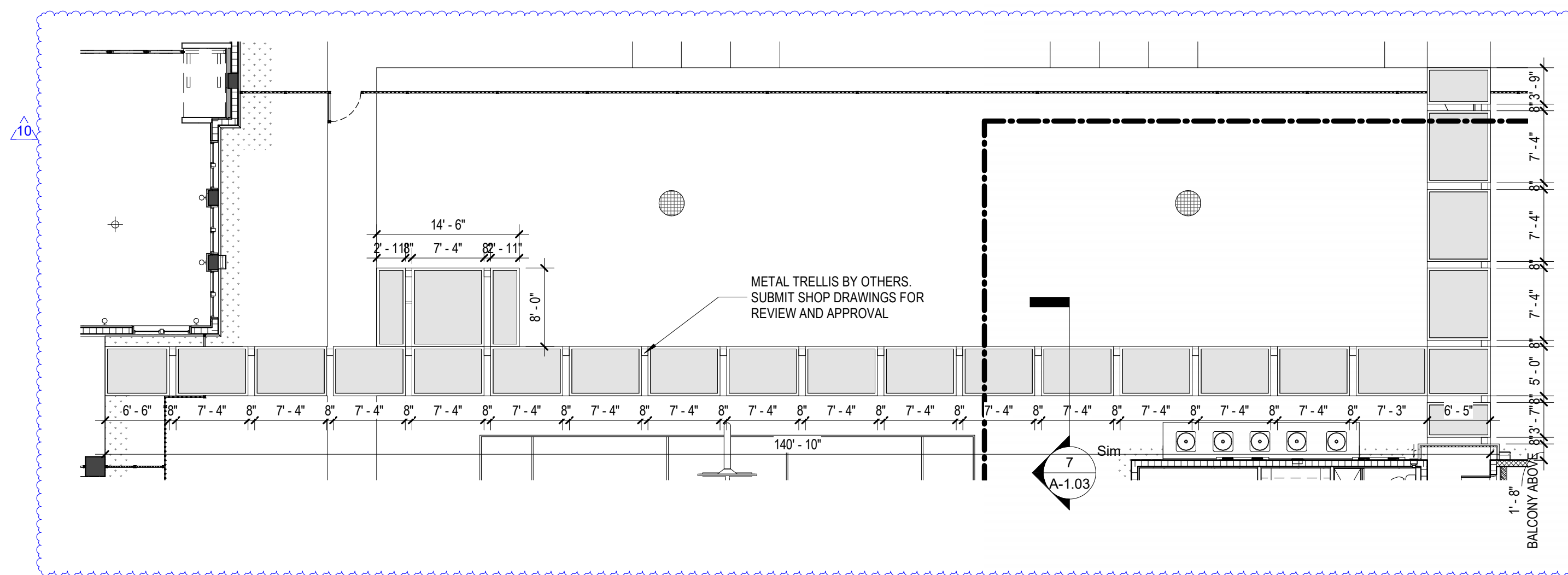
4 TYP. WALL FEATURE SCALE: 3/8" = 1'-0" RESIDENTIAL BUILDING
