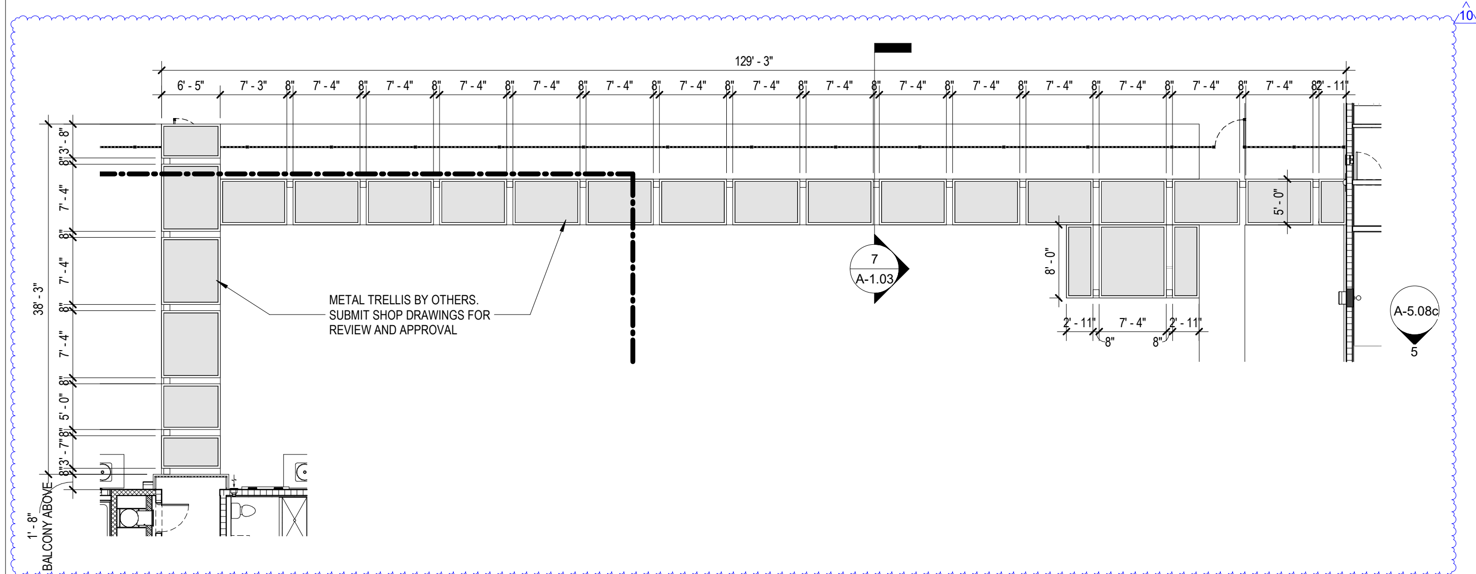
5 ENLARGED TRELLIS DETAIL SCALE: 3/32" = 1'-0"
