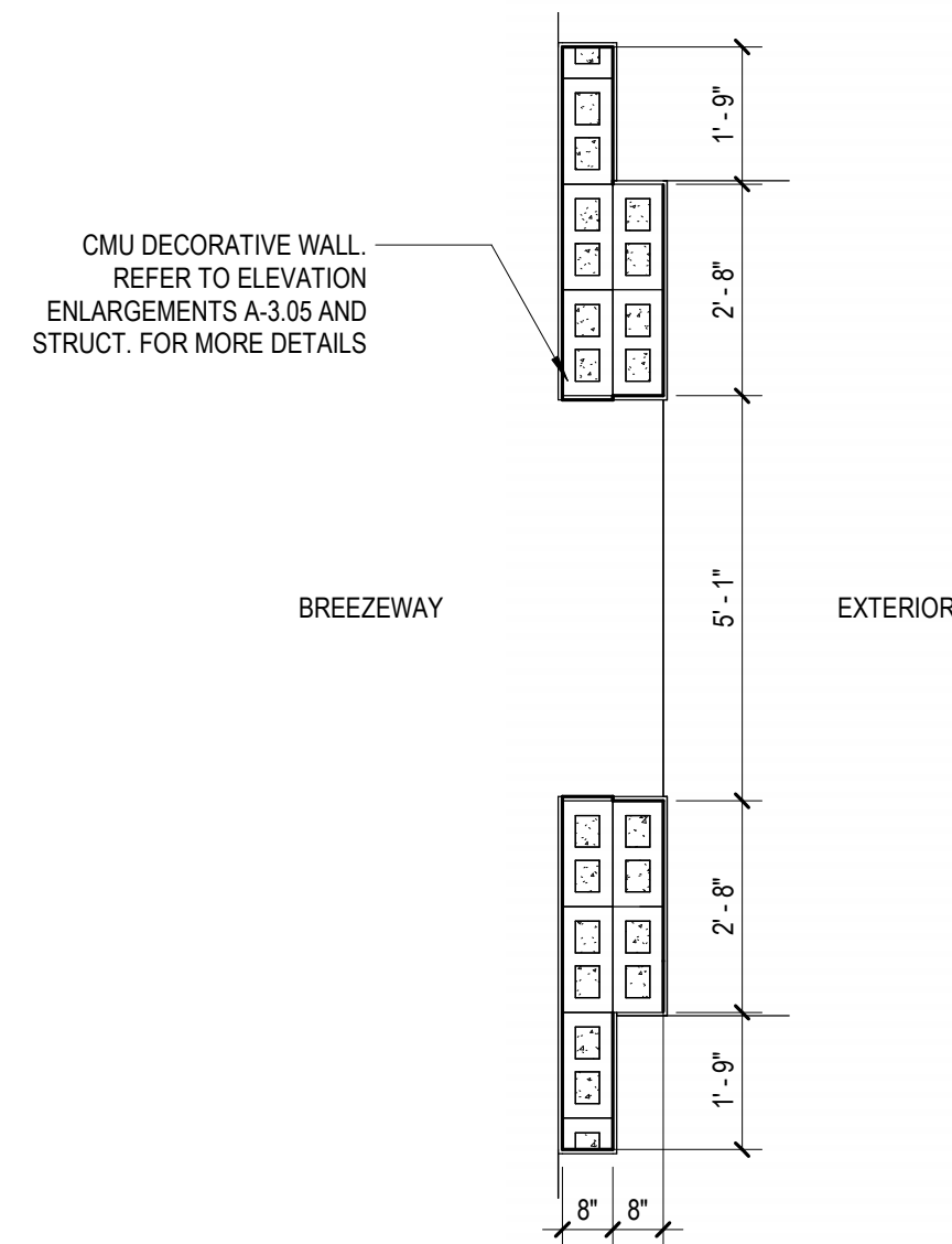
3 TYP. WALL FEATURE SCALE: 3/8" = 1'-0" RESIDENTIAL BUILDING
