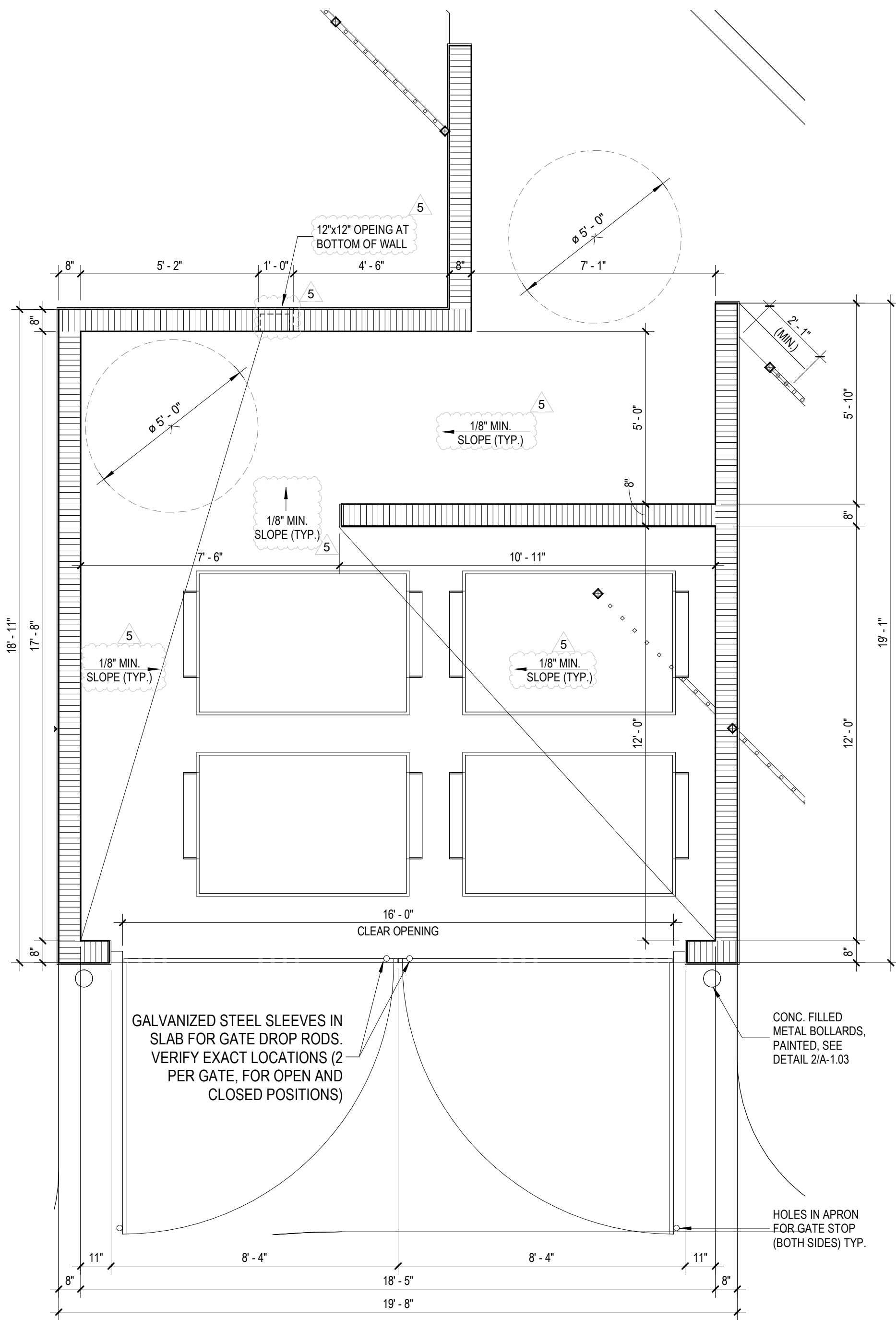
1 COMMUNITY CENTER TRASH ENCLOSURE SCALE: 3/8" = 1'-0"
